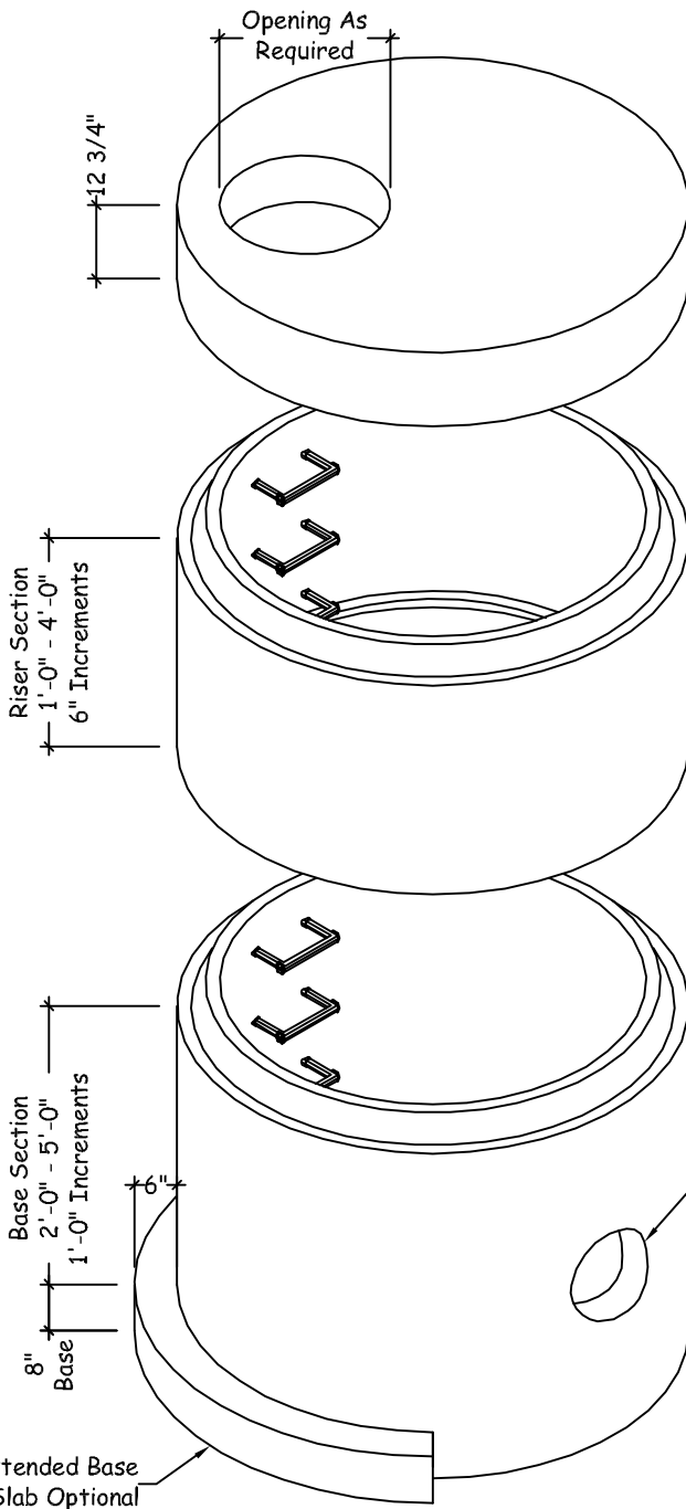
Isometric View
