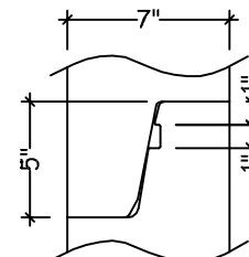
Joint Detail
