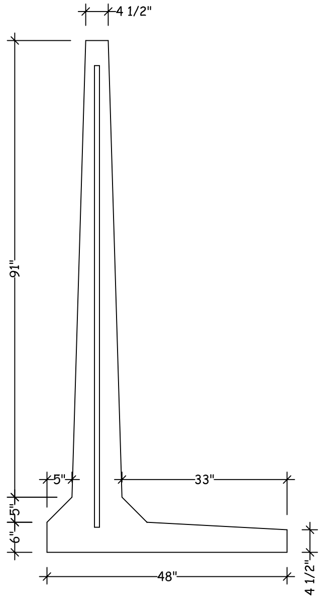
End View
