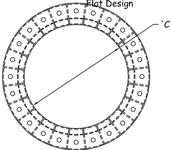
Polyethylene Grade Ring Flat Design
