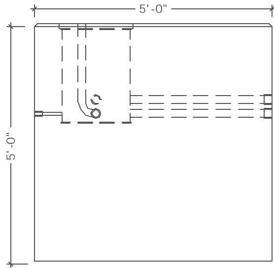
ELEVATION VIEW 'B'
