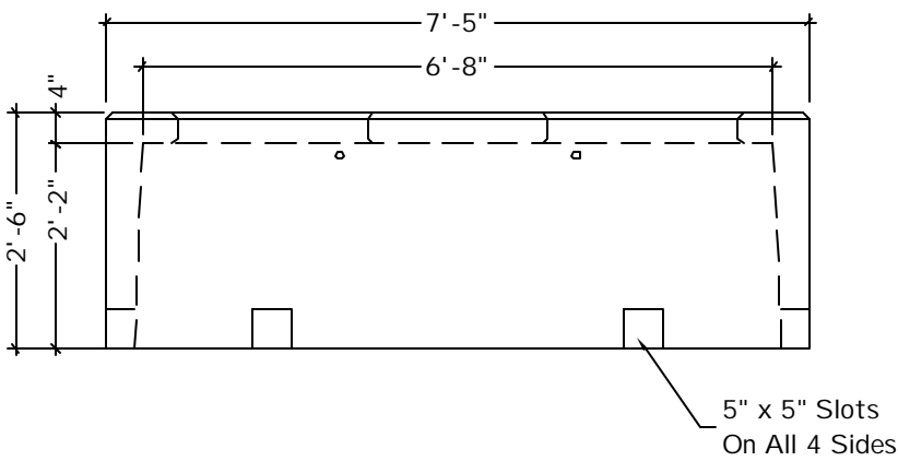
SECTION VIEW 'A'
