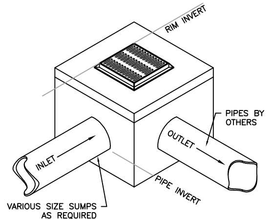
IN-FIELD VIEW
