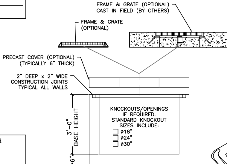
ELEVATION VIEW
