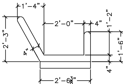
ELEVATION VIEW
